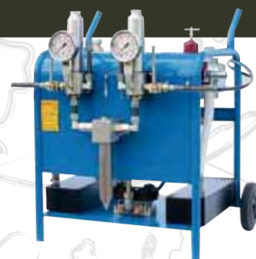
Pompa bicomponente a soffietto Bellows Pump for two component
